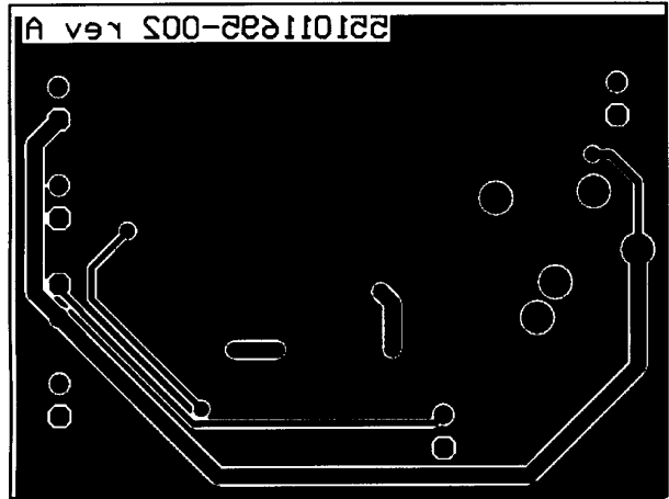
FIGURE 7. Bottom Layer
