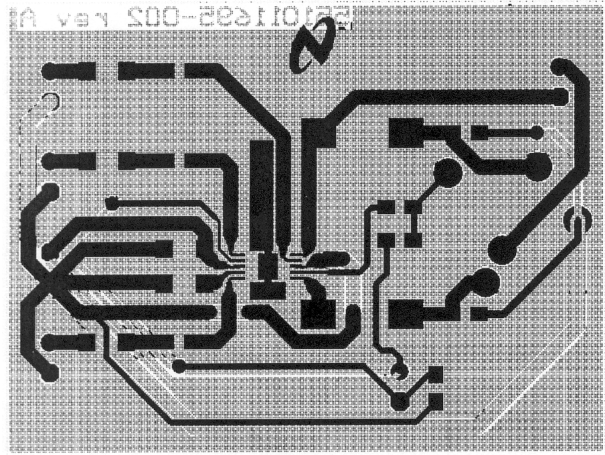
FIGURE 8. Composite Layer
